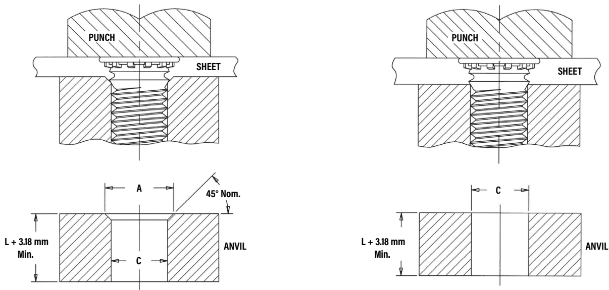
Tooling for sheet thicknesses less than 1.51 mm with M2.5 thru M5 thread sizes and less than 2.36 mm for M6 threads.
