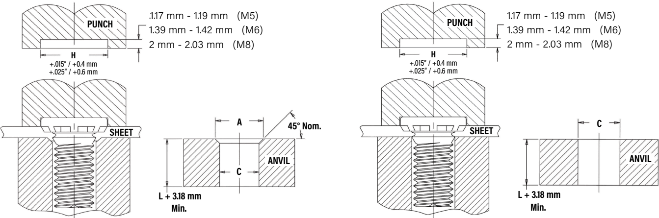
Tooling for sheet thicknesses less than 1.51 mm with M5 and M6 thread sizes and less than 1.9 mm with M8 threads.
